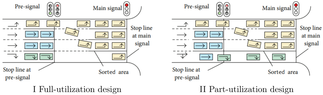
Figure 2.2. – Pre-Signal Classification Based on Sorted Area Utilization, Adapted from (Li et al., 2014)
