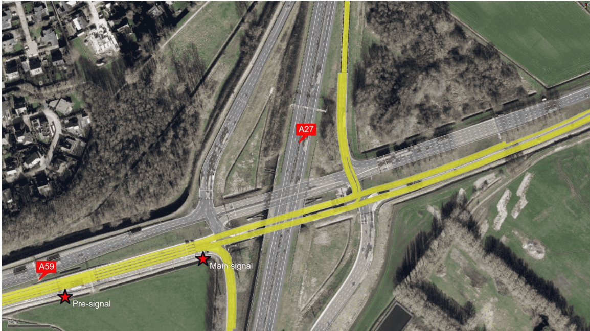
Figure 5.8. – Range of Traffic Directions for the West-East A59 Pre-Signal
