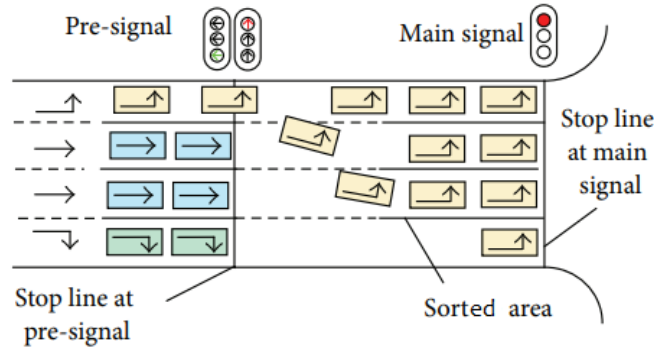
Figure 1. – Example of the Pre-Signal's Working Mechanism (Li et al., 2019)
