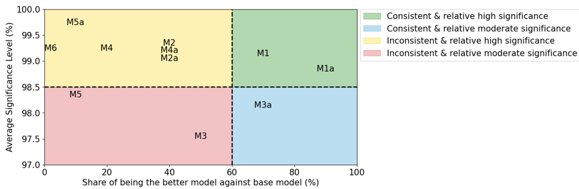
Figure 7.10. – Adapted Form of Figure 7.9: Relaxation of the Significance Level From 95% to 80% for the Additional Parameter(s) Being Different From Zero
