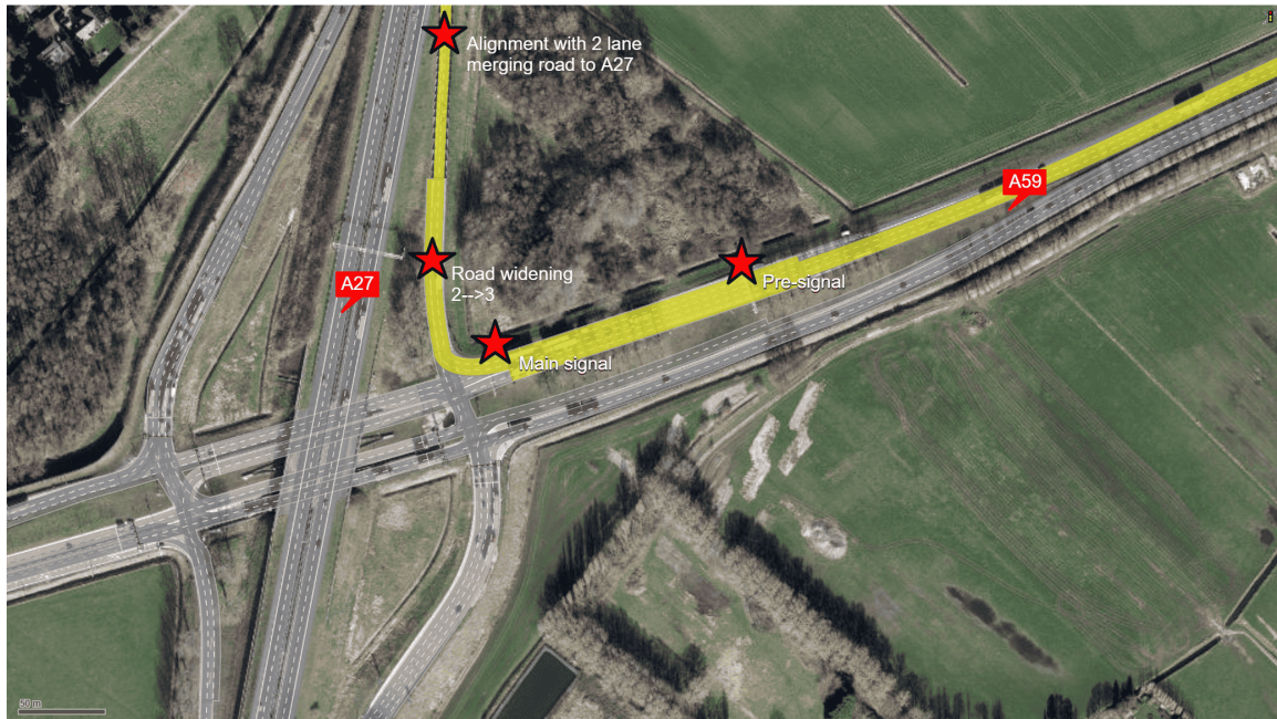
Figure 5.6. – Road Section That Facilitates a Pre-Signal System Size of 3 Lanes in Right-Turning Direction
